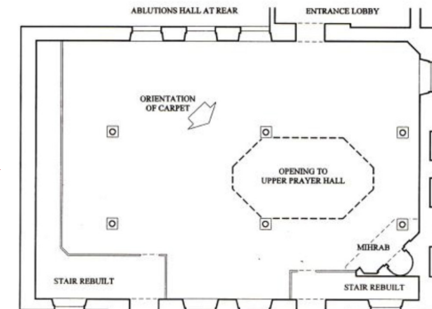
Fig. 26 - Floor plan of London Jamme Masjid (Great Mosque) 1976 as remodelled in 1986-87
